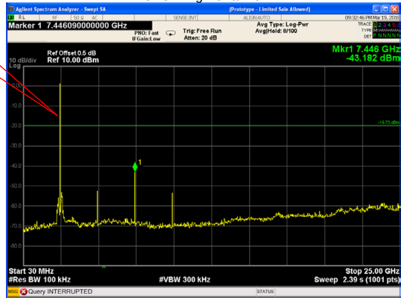
GFSK High Channel
