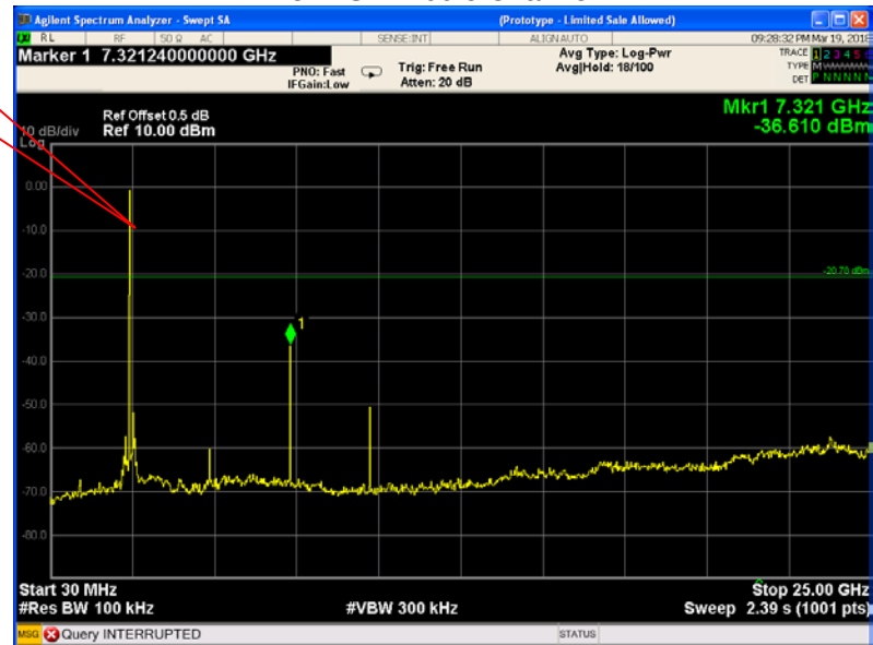
8DPSK Middle Channel
