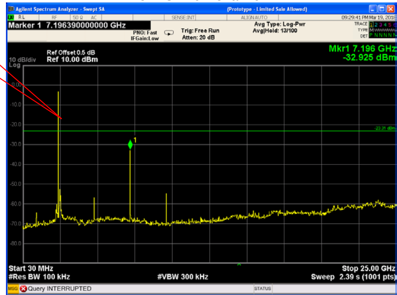
8DPSK Low Channel
