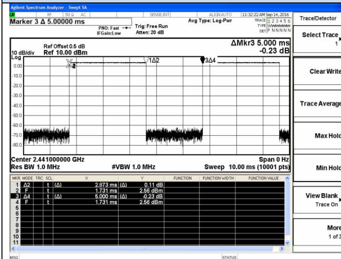
DH5-2441MHz
