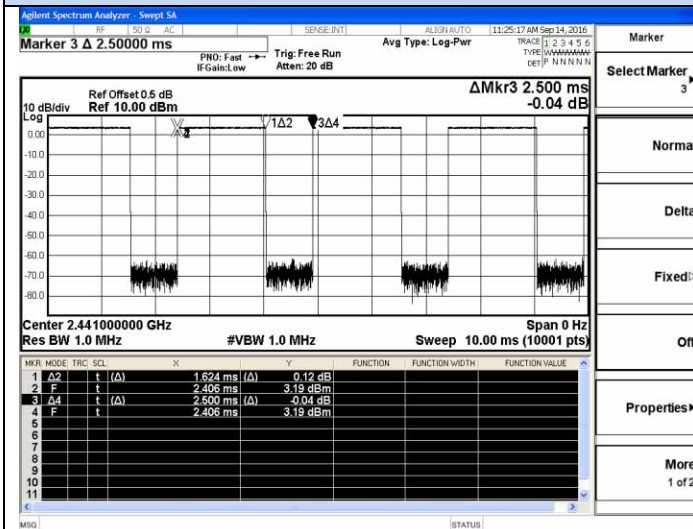
DH3-2441MHz
