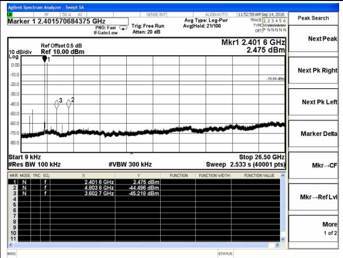
DH1-Low channel
