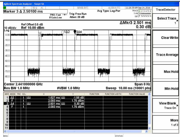
2DH3-2441MHz
