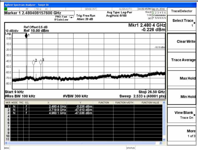
3DH1-High channel
