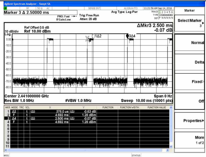
2DH1-2441MHz
