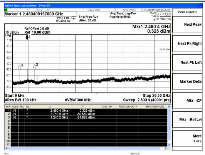
2DH1-High channel
