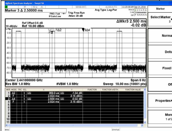
DH1-2441MHz
