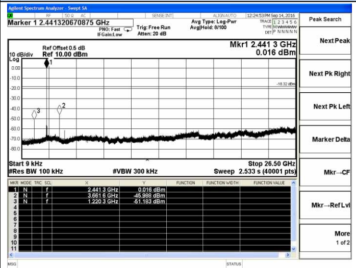
2DH1-Middle channel
