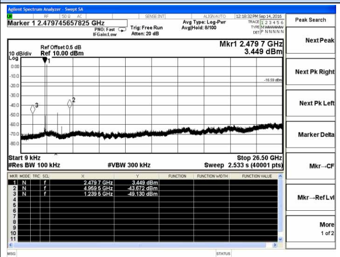
DH1-High channel
