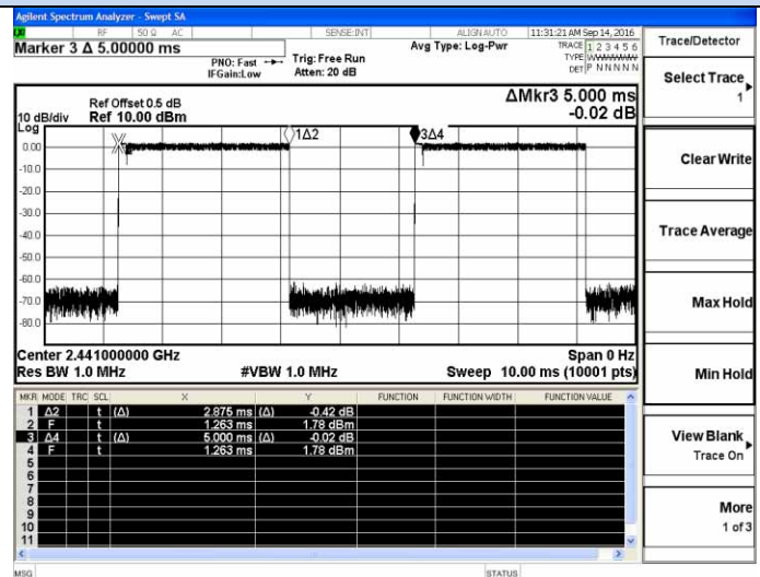
2DH5-2441MHz
