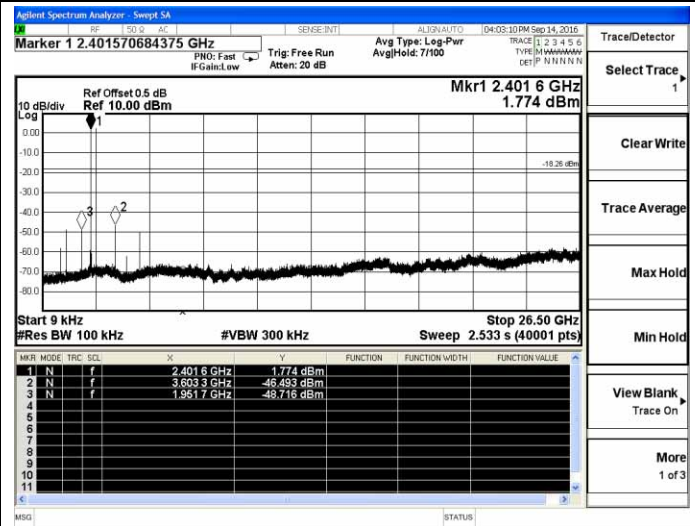
3DH1-Low channel
