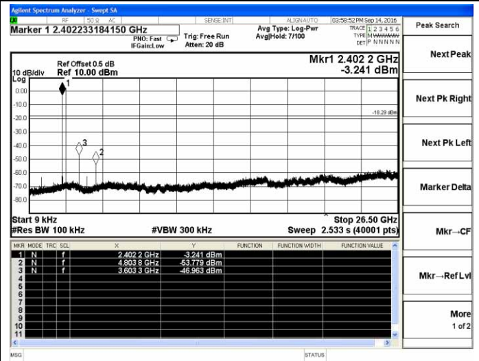
2DH1-Low channel
