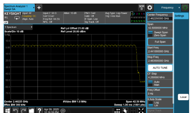
3-DH5(3Mbps)-2441~2483.5MHz
