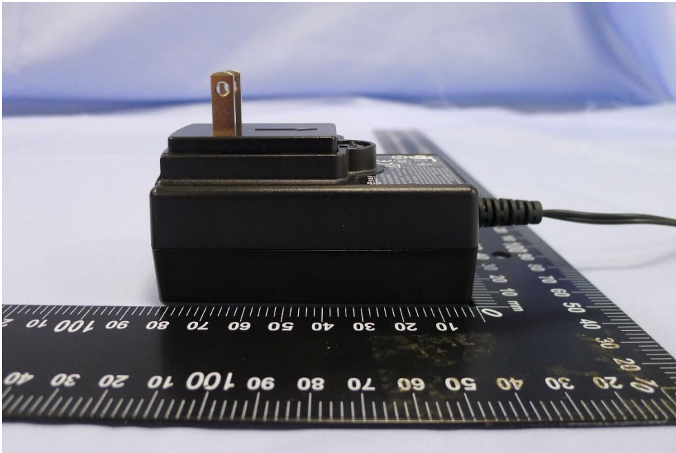
(12) Adapter Photo
