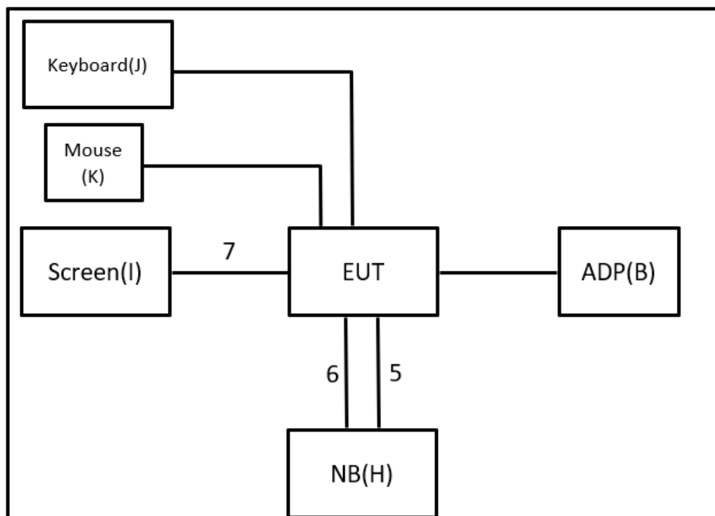
Radiated Emissions
