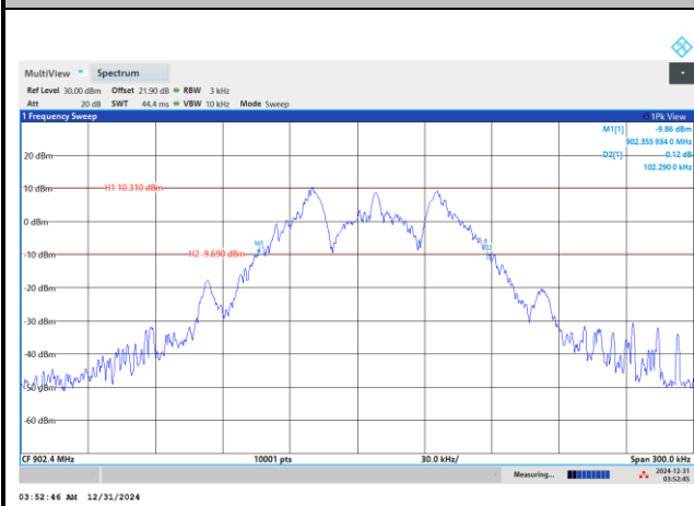
20 dB Bandwidth Plot in 902.4MHz
