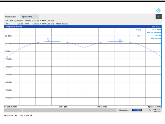
Channel Separation Plot on Channel 915.2MHz
