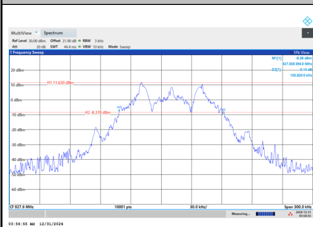
20 dB Bandwidth Plot in 927.6MHz
