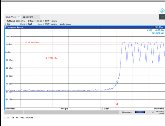
Hopping Mode Low Band Edge Plot
