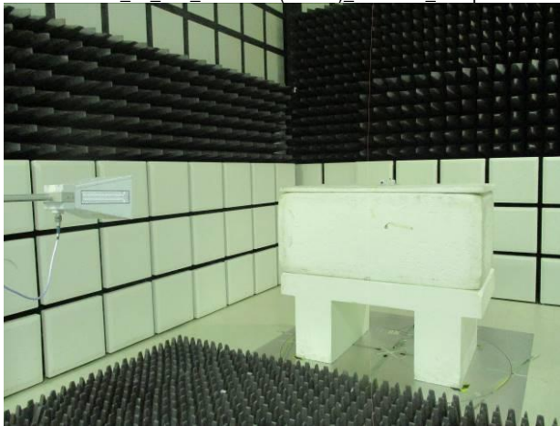
FCC_15_247_LRF_Radiated_Setup
