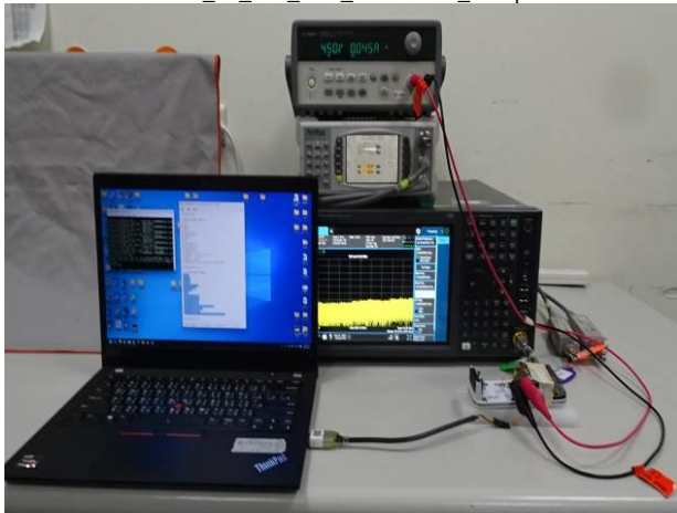
FCC_15_247_802.11ah (OFDM)_Conducted_Setup
