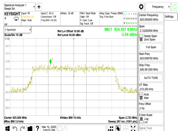
PSD_OFDM 2M_HighCH-925MHz
