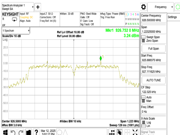
PSD_OFDM 1M_HighCH-926.5MHz
