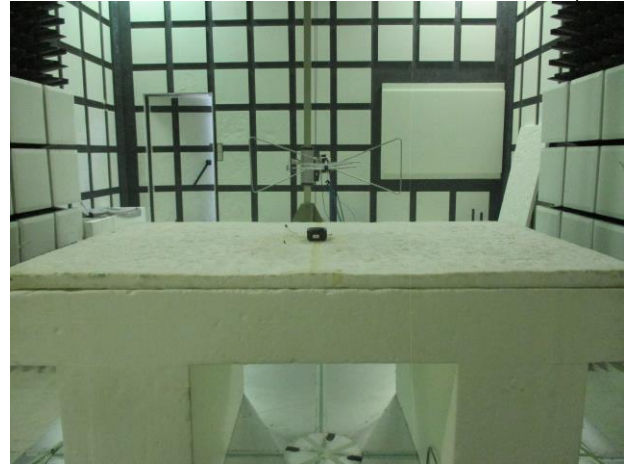
FCC_P15_247+IC_RSS_247_900M_OFDM_Radiated_Setup
