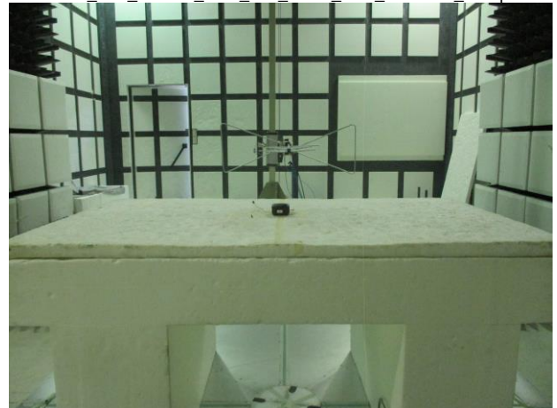
FCC_P15_247+IC_RSS_247_900M_FSK_Radiated_Setup
