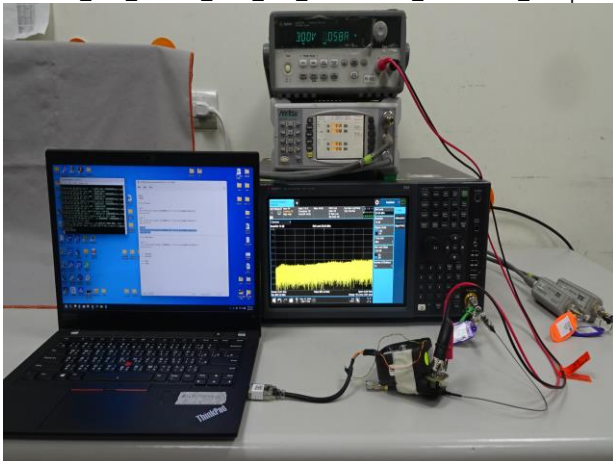
FCC_P15_247+IC_RSS_247_WLAN 2.4G_Conducted_Setup
