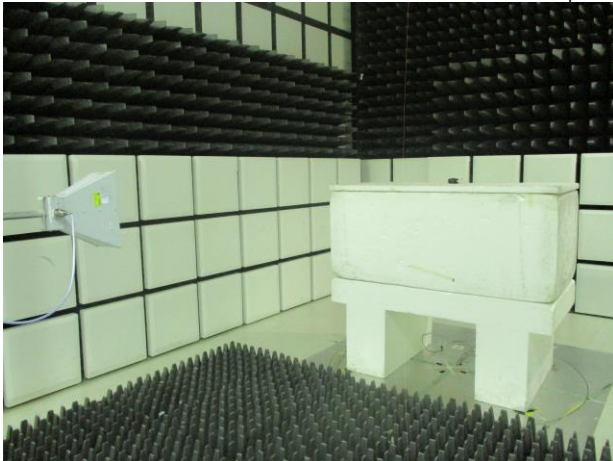
FCC_P15_247+IC_RSS_247_900M_OFDM_Radiated_Setup
