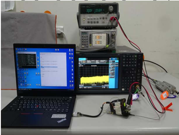
FCC_P15_247+IC_RSS_247_WLAN 2.4G_Conducted_Setup
