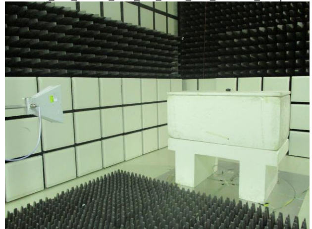
FCC_P15_247+IC_RSS_247_900M_FSK_Radiated_Setup
