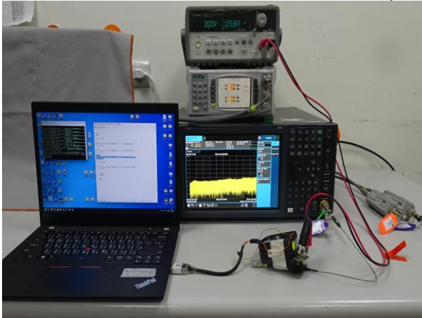
FCC_P15_247+IC_RSS_247_900M_OFDM_Conducted_Setup
