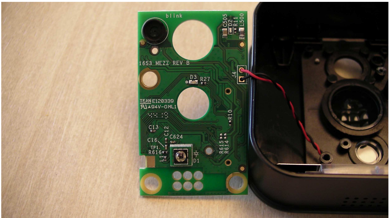
Mezz Board Side 2
