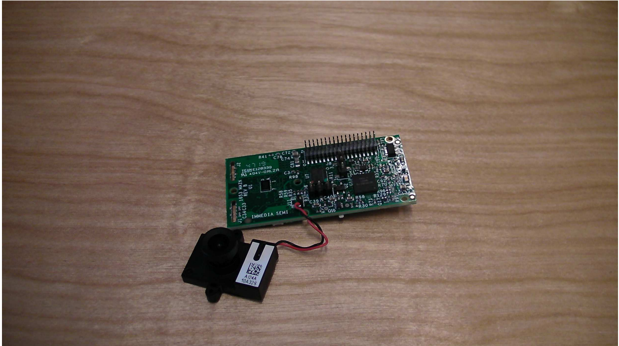
Main Board with Camera PIR Board Removed, Battery /Antenna Board Detached
