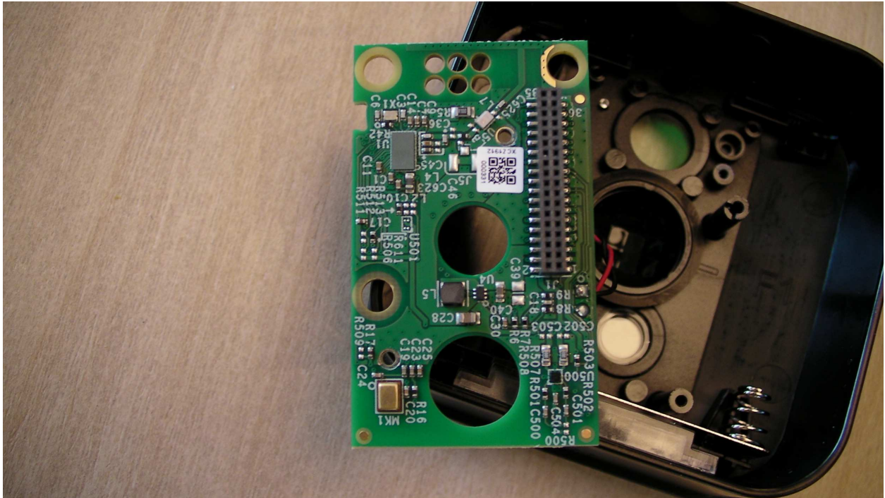
Mezz Board Side 1
