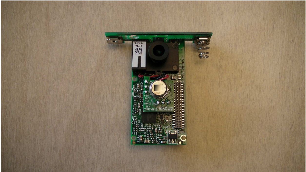
Main Board with Camera PIR Board, Battery /Antenna Board Attached
