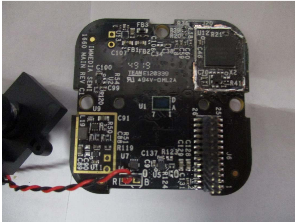
Main Board Side 2 Camera Shutter & RF Enclosure Removed
