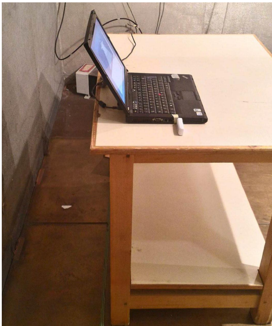
Conducted emission measurements (side view)
