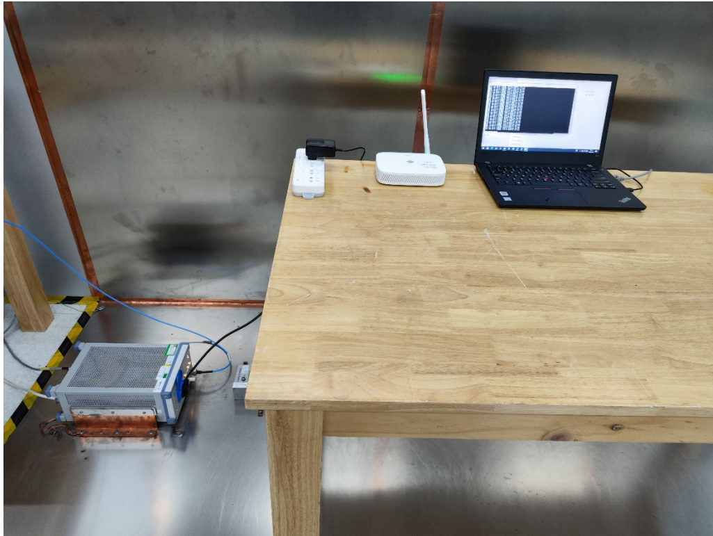
Photograph 1: Set-up for Conducted Emissions, AC Mains
