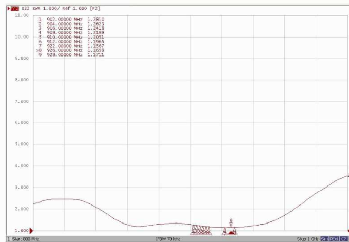
Figure 2: RAKARG15 VSWR graph
