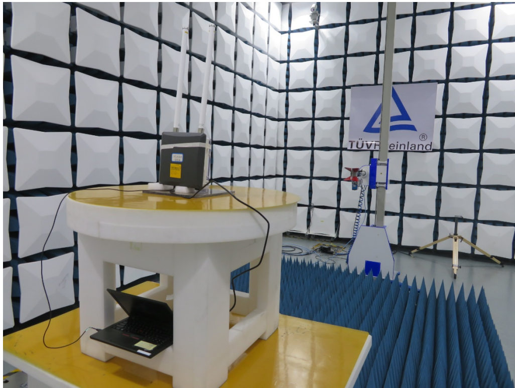
Photograph 5: Set-up for Radiated Spurious Emission, above 1GHz
