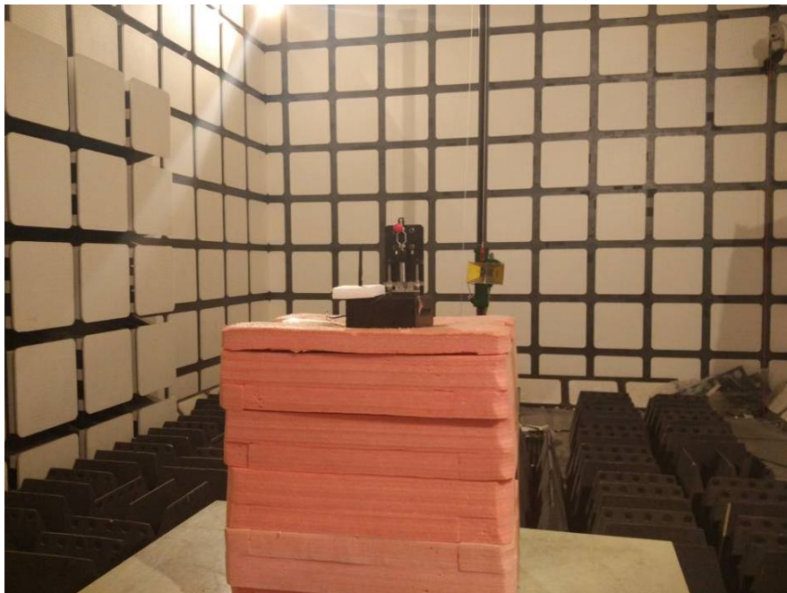
Radiated Emissions View – External Antenna (Above 1 GHz)
