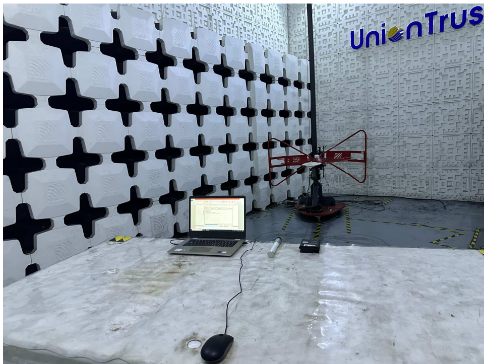
Photograph 1: Set-up for Radiated Spurious Emissions
