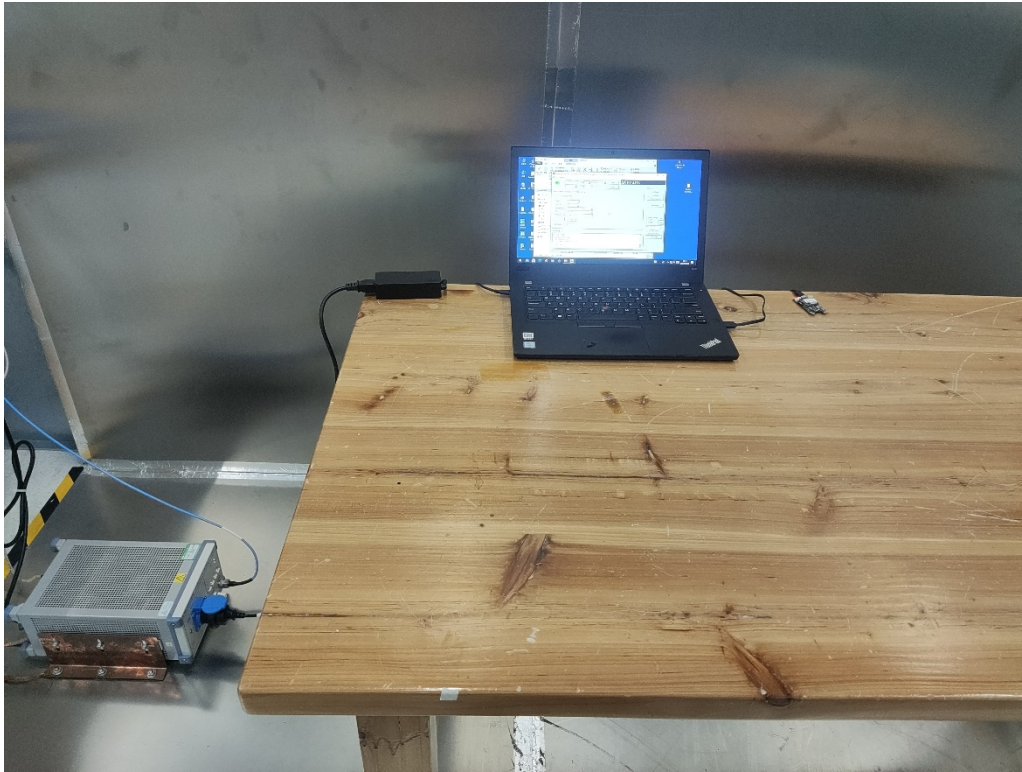
Photograph 3: Set-up for Conducted Emissions ON AC mains
