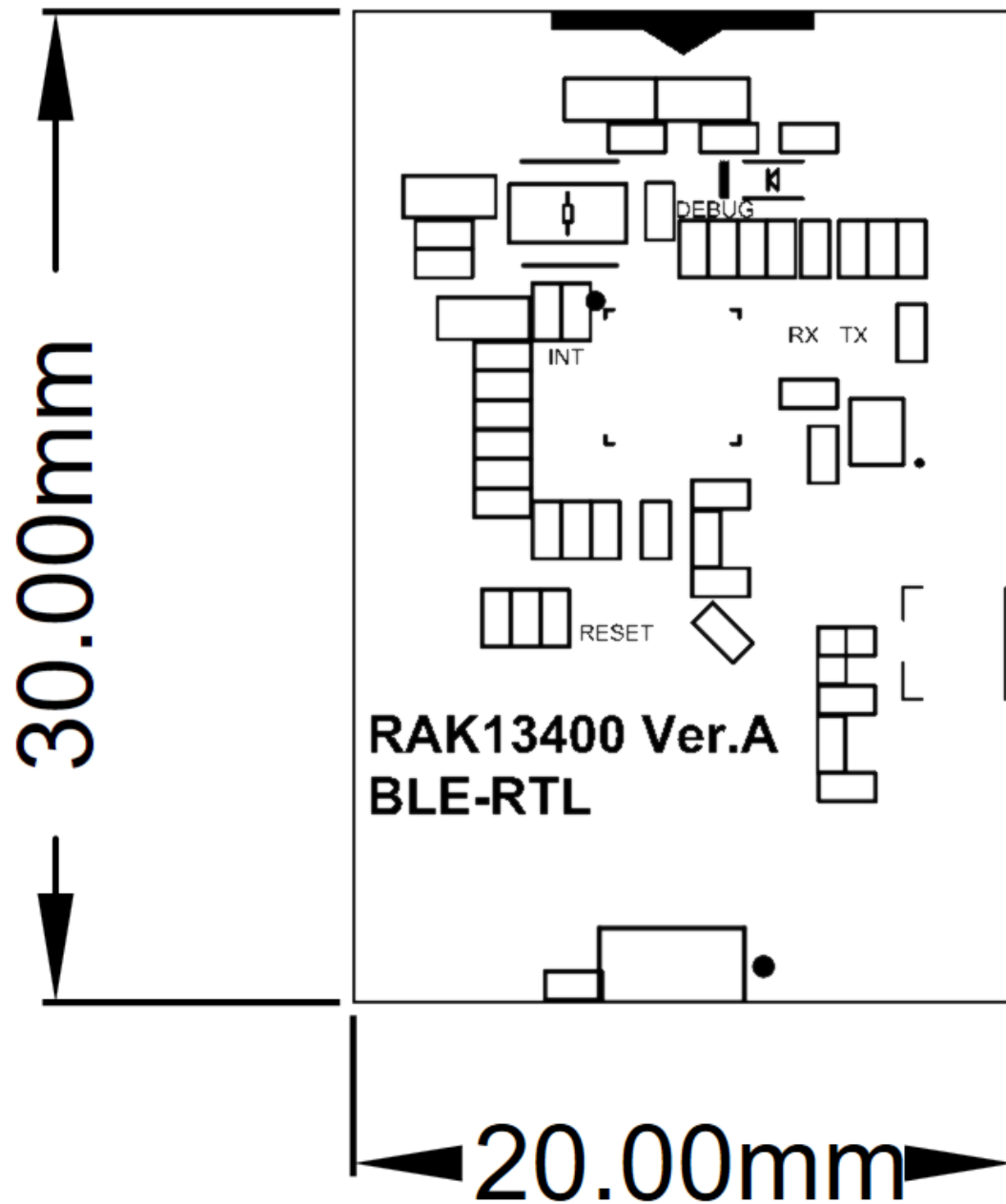
Figure 3: RAK13400r Module Mechanic Drawing
