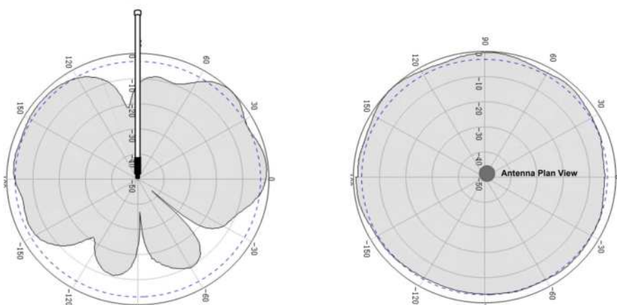
Figure 4: RAKARG12 Radiation Pattern for 870 MHz
