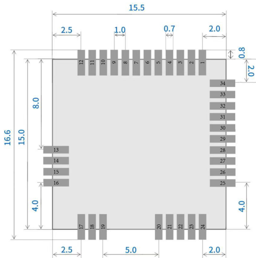
Figure 4: RAK11720 Layout
