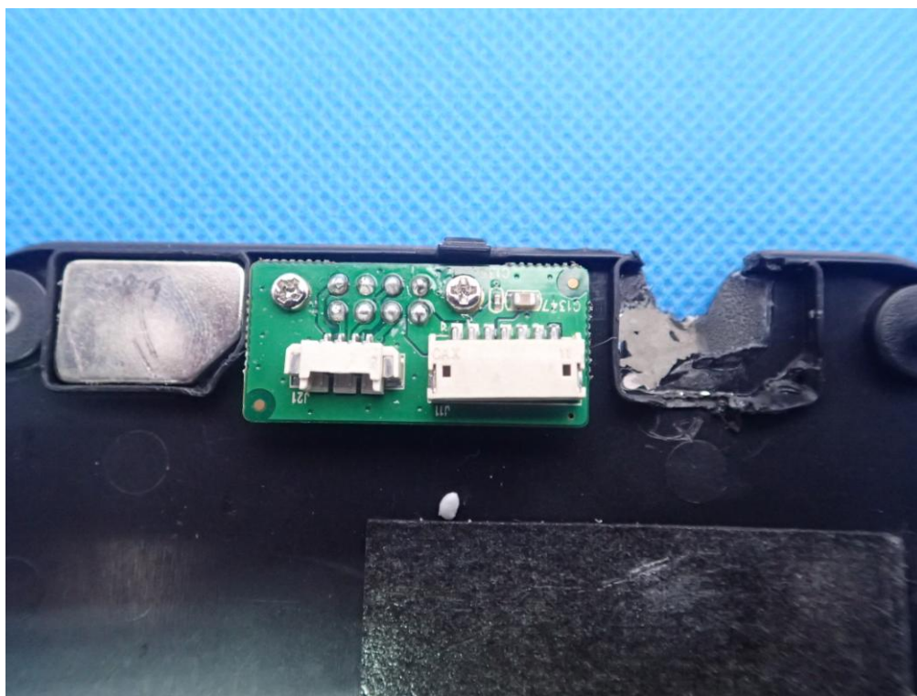
INTERNAL VIEW OF Battery Back-Up -5
