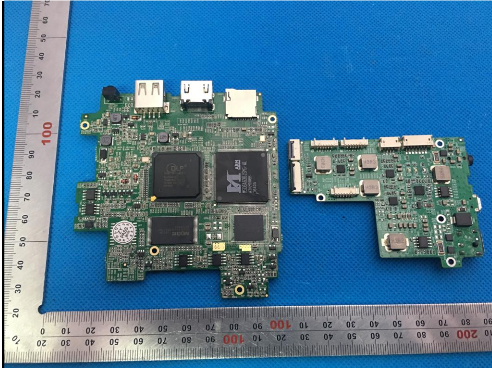
INTERNAL VIEW OF Projector -1
