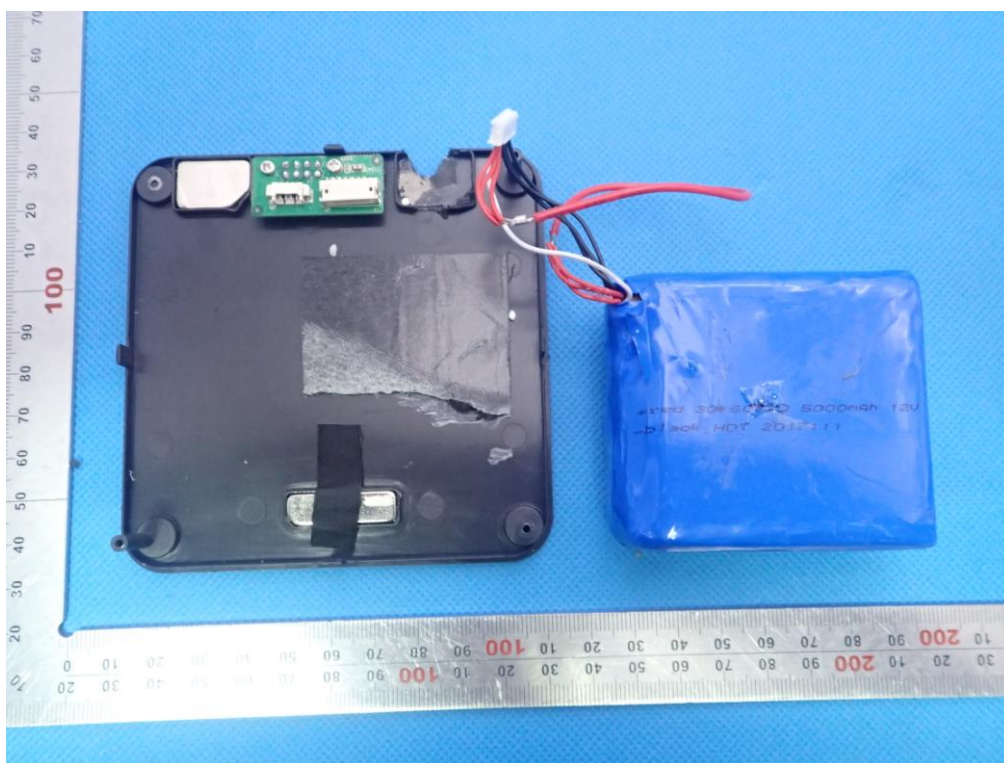
INTERNAL VIEW OF Battery Back-Up -3
