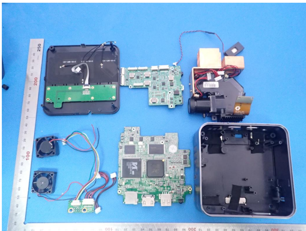
OPEN VIEW OF Projector 2
