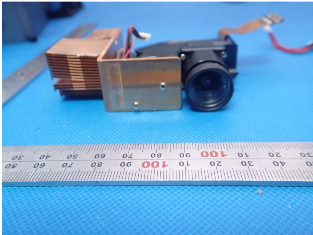
OPEN VIEW OF Projector 4
