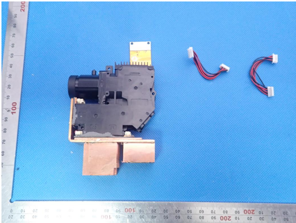
OPEN VIEW OF Projector 6
