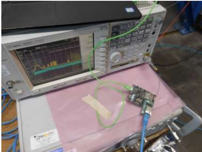
Power Setup
