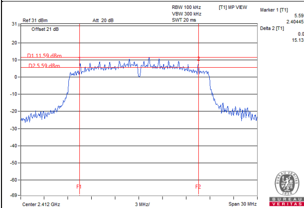
VHT20_Chain 2 / CH1
