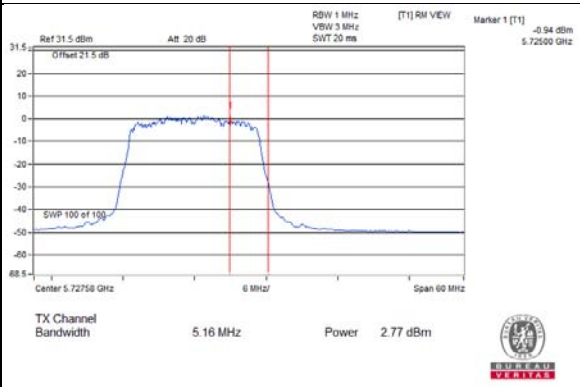
802.11ac (VHT20)_Chain 2 / CH144 (U-NII-3 Band)
