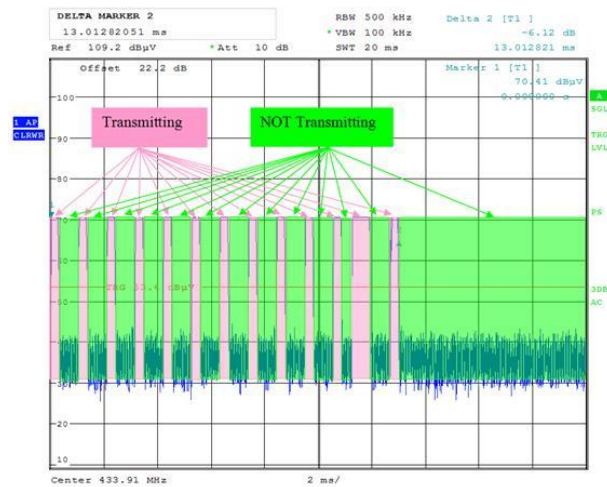
Figure 8.2-2: Pulse width
