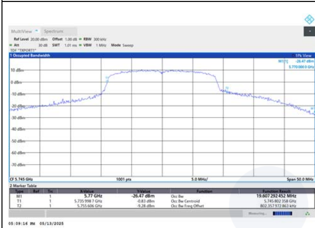
UNII 3 / 802.11ac VHT 20 / Low ch.
