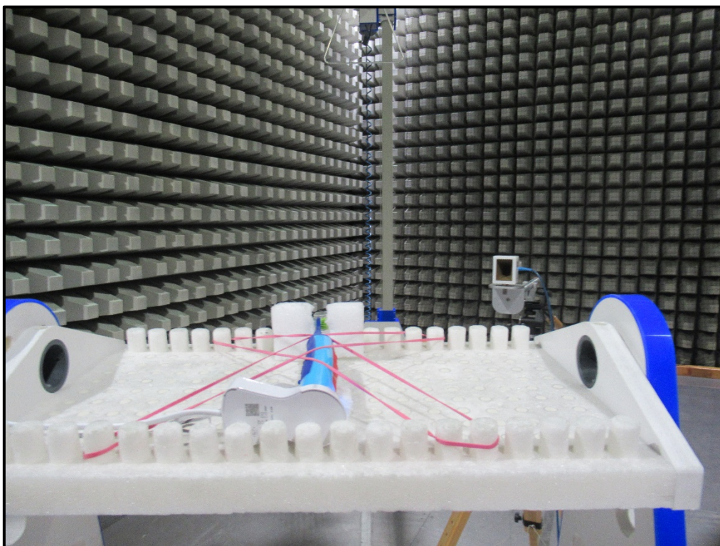
Photo 9: Radiated Test Setup-18 GHz – 25 GHz
