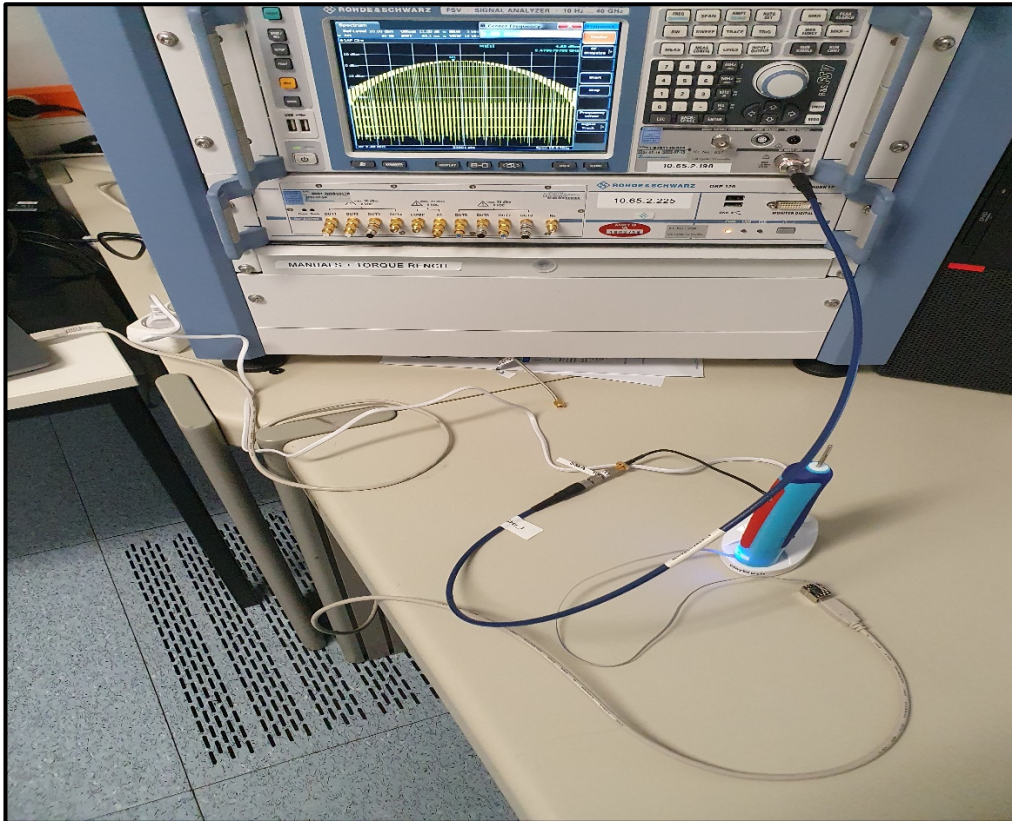
Photo 10: Conducted Test Setup
