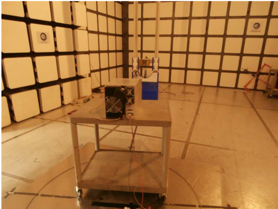
Radiated Emissions 1 GHz to 5 GHz
