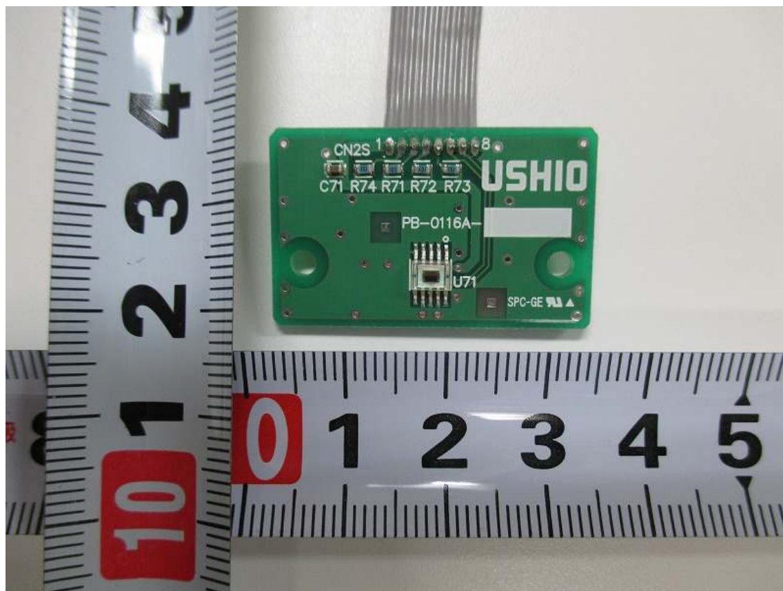
PCB:PB-0116A
