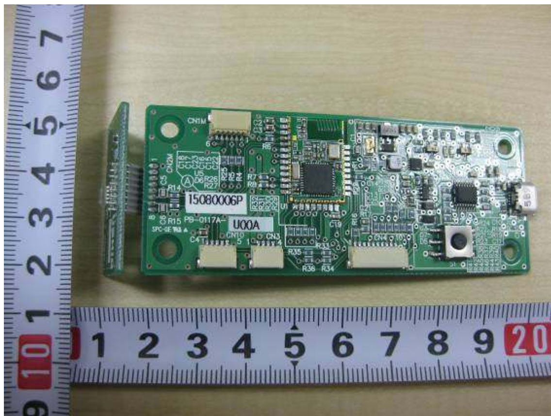
PCB:PB-0117A
