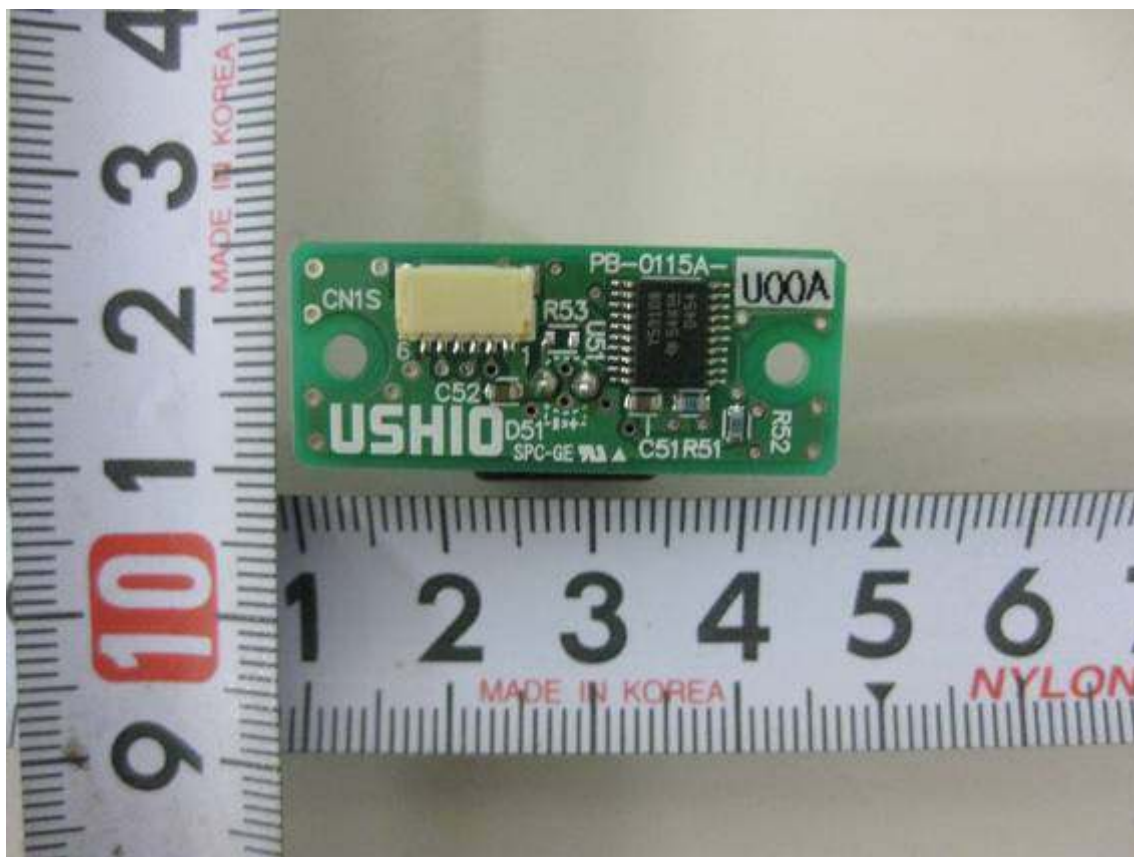
PCB:PB-0115A
