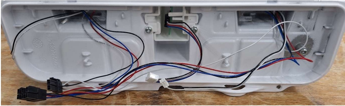
Photo 4 - internal view 4 (detail)
