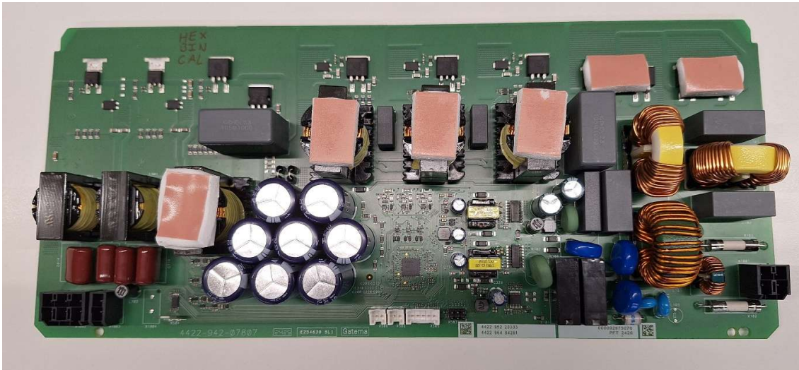
Photo 7 – Main board top
