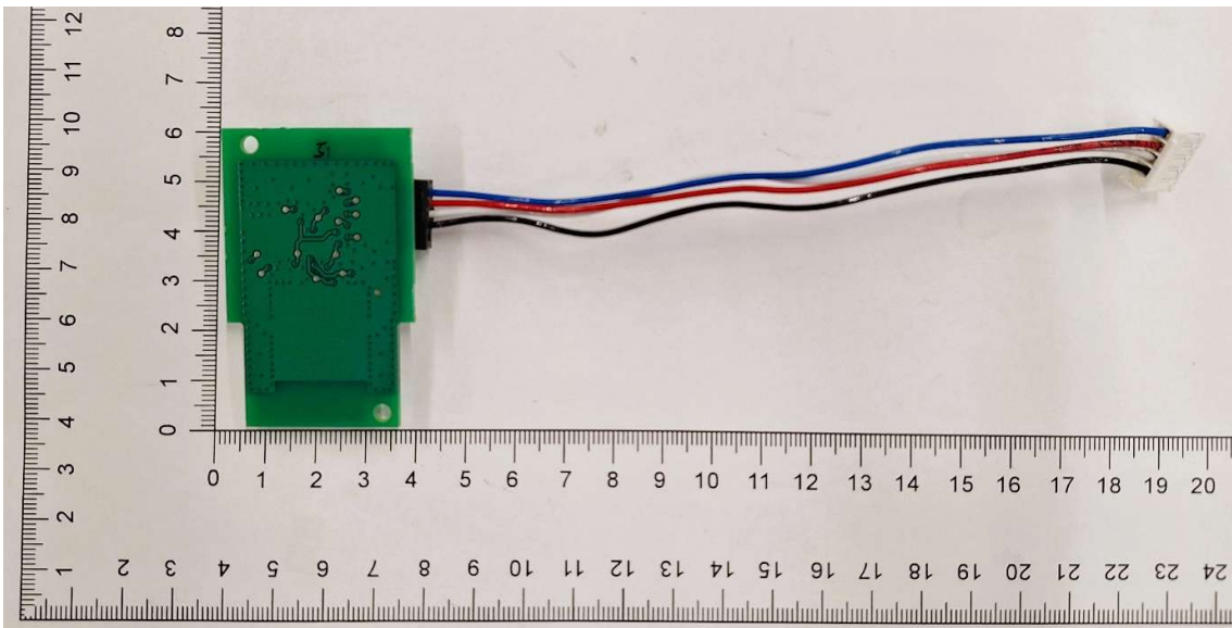
Photo 6 – Radio board bottom
