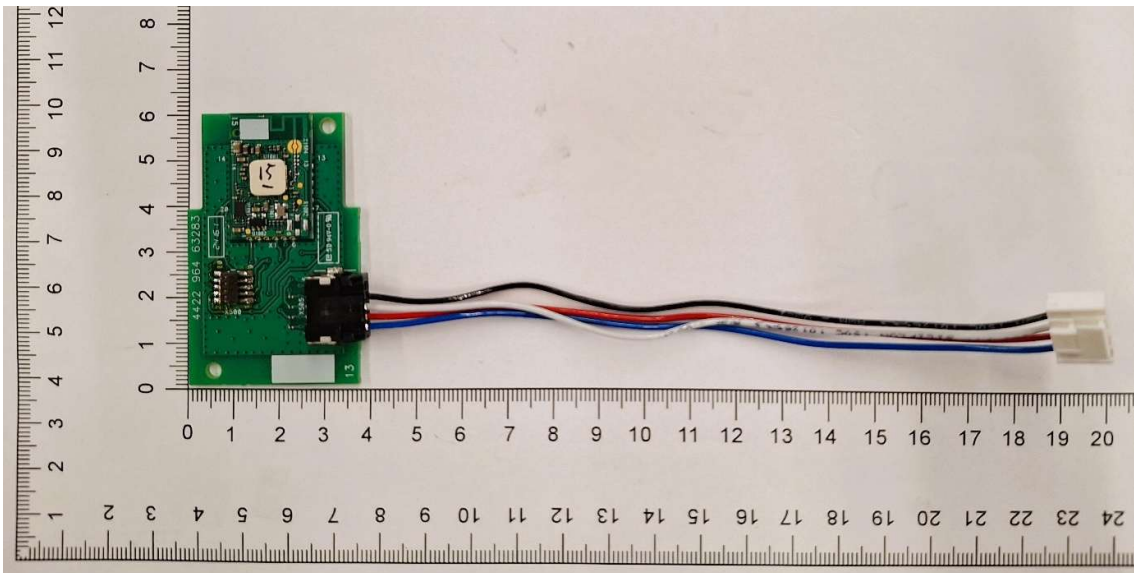
Photo 5 – Radio board top
