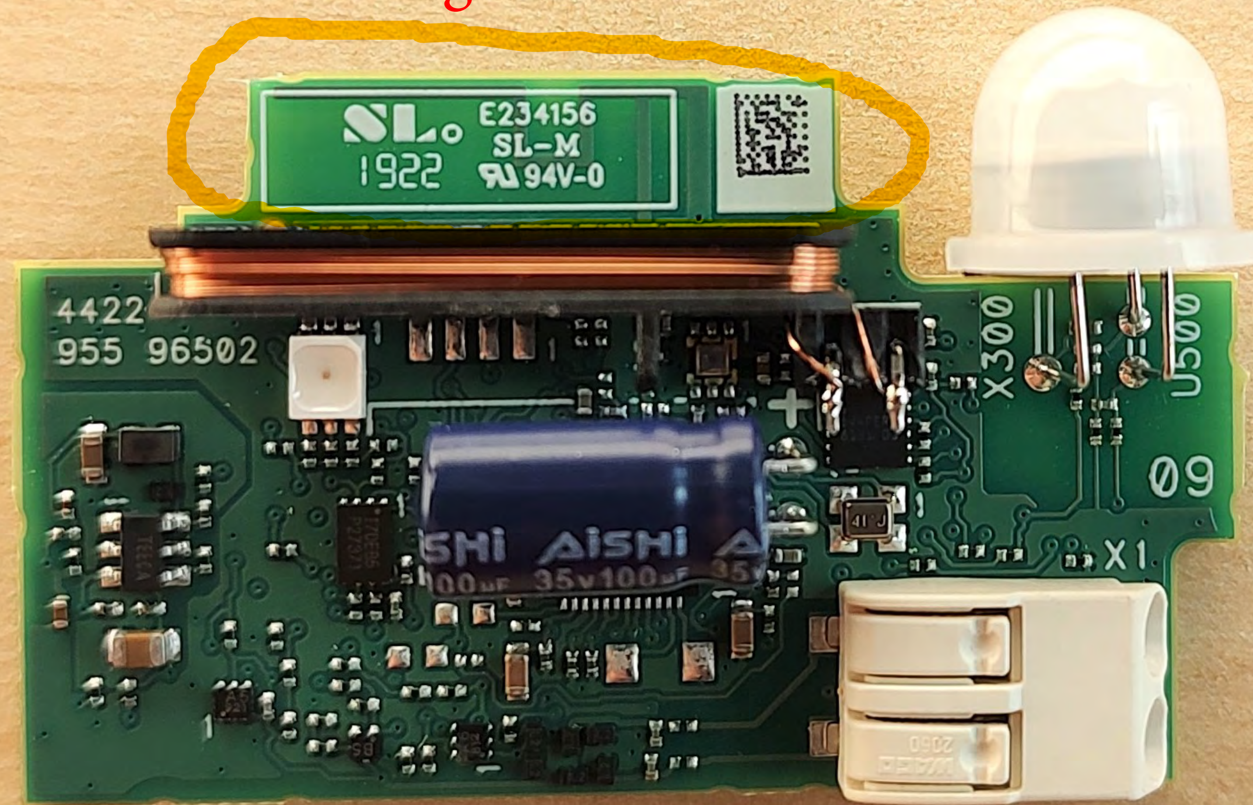
BT & Zigbee Antenna
