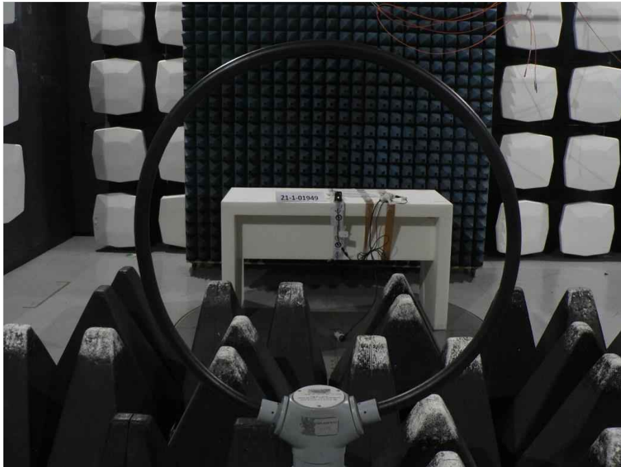
Photograph 3: EUT test setup in the semi anechoic chamber, overview_EUT elevation 90°
