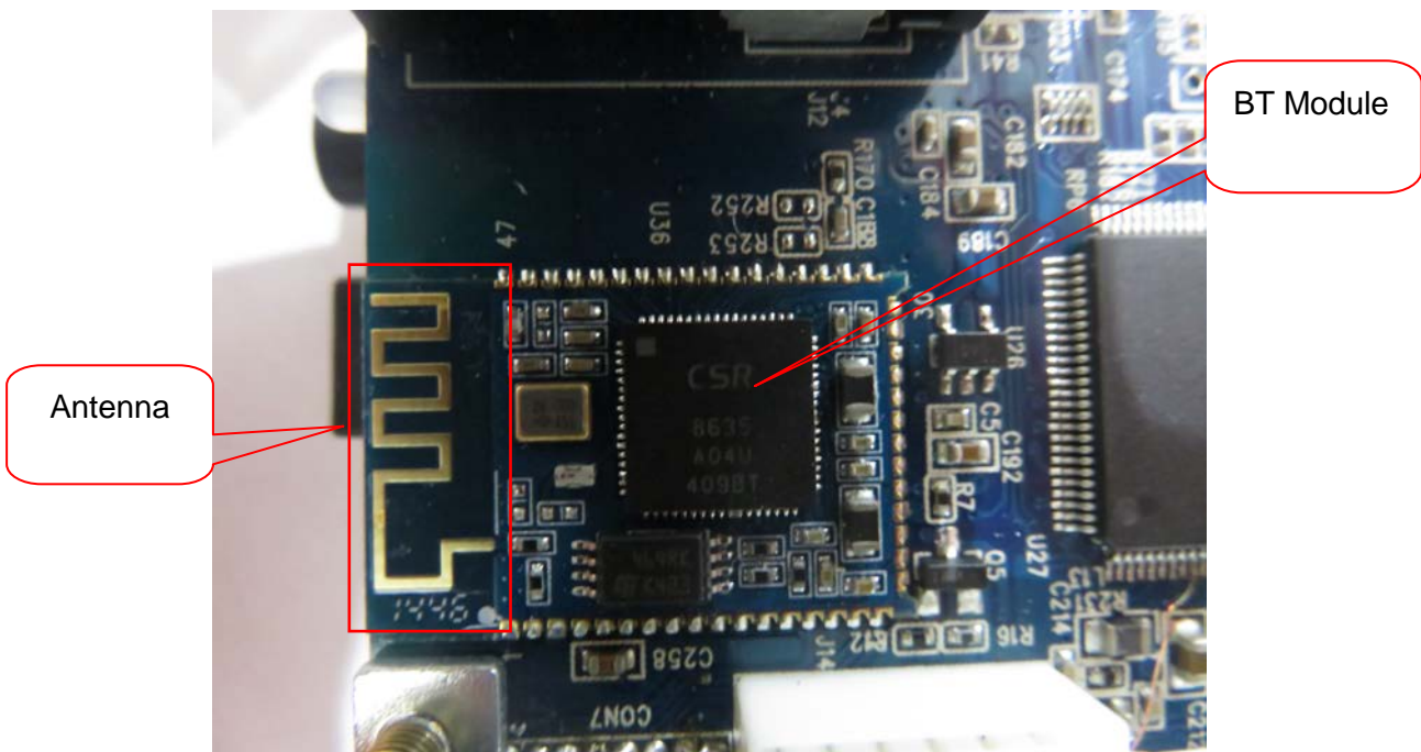
View of the Bluetooth module
