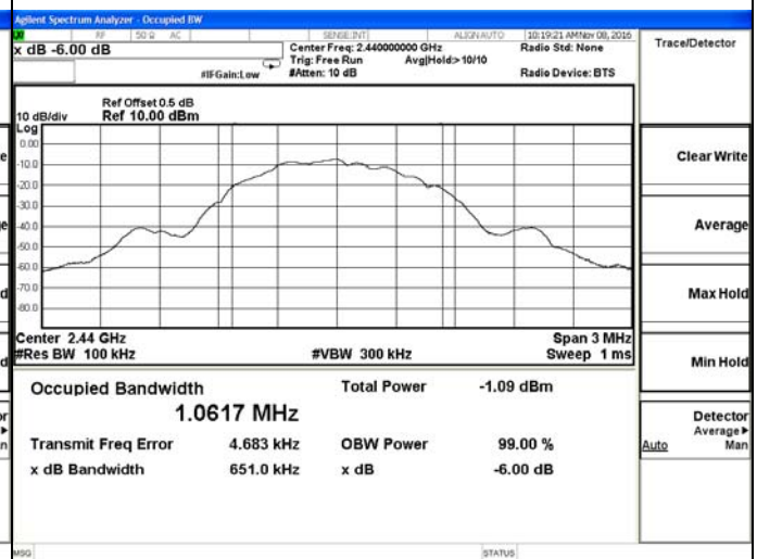
Channel 19 / 2440 MHz
