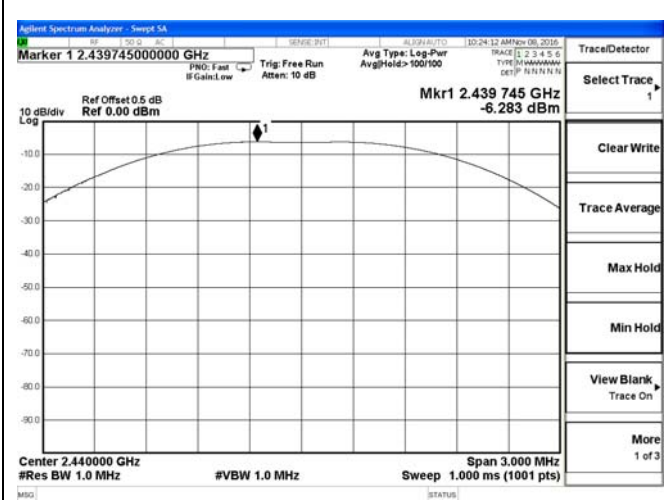
Channel 19 / 2440 MHz
