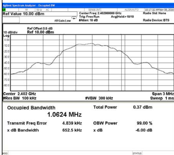
Channel 0 / 2402 MHz
