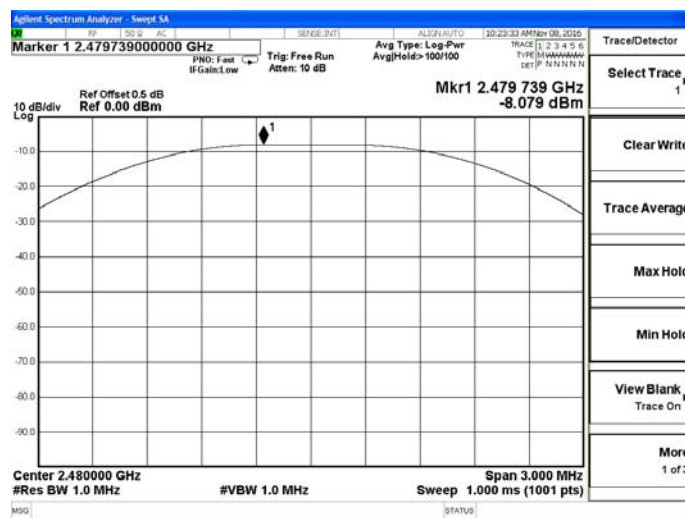
Channel 39 / 2480 MHz
