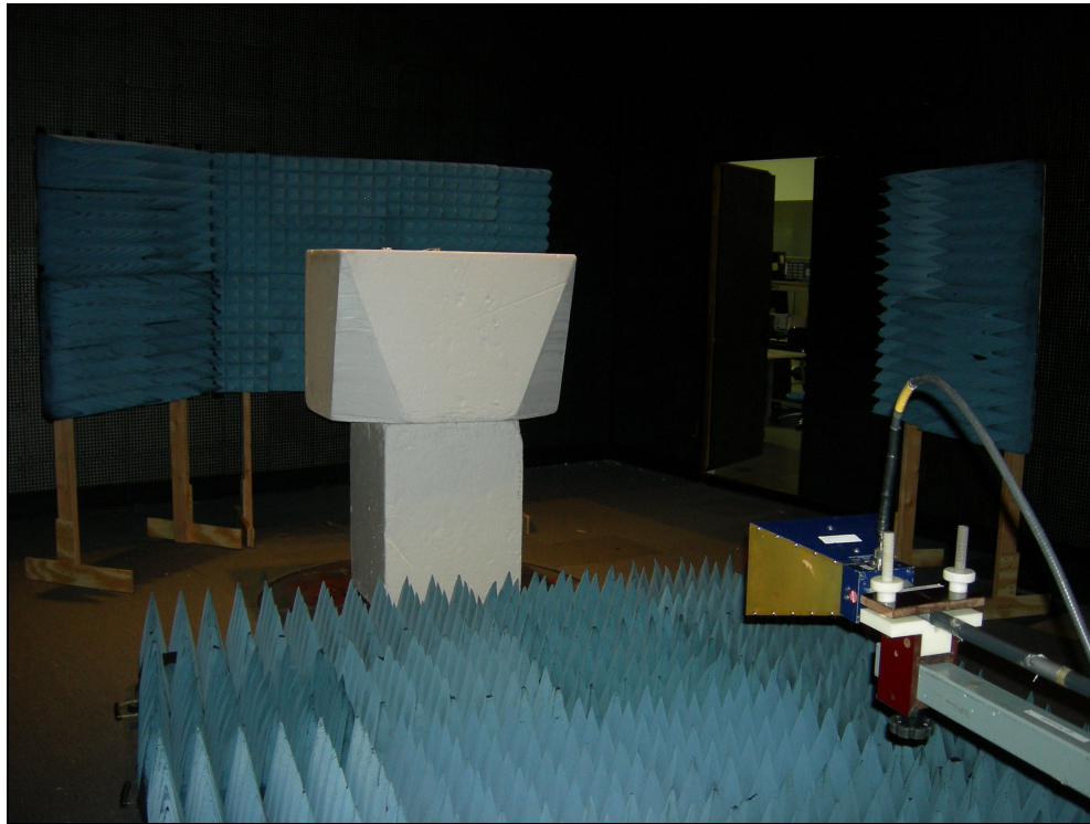
Figure 1: Test Setup Photo – Radiated Emissions XPOS
