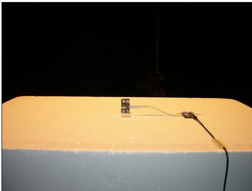
Figure 4: Test Setup Photo – Radiated Emissions YPOS
