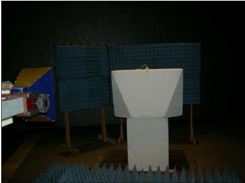
Figure 5: Test Setup Photo – Radiated Emissions ZPOS
