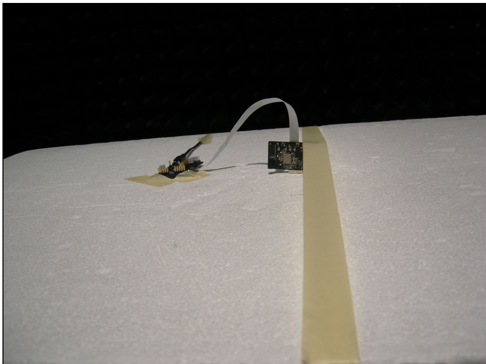
Figure 6: Test Setup Photo – Radiated Emissions ZPOS
