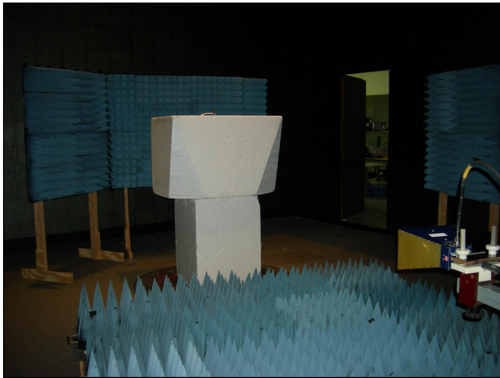
Figure 3: Test Setup Photo – Radiated Emissions YPOS
