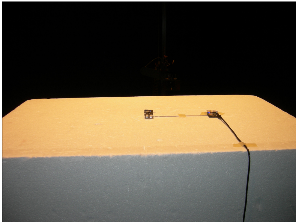
Figure 2: Test Setup Photo – Radiated Emissions XPOS
