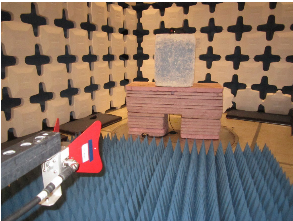
1GHz-6GHz
