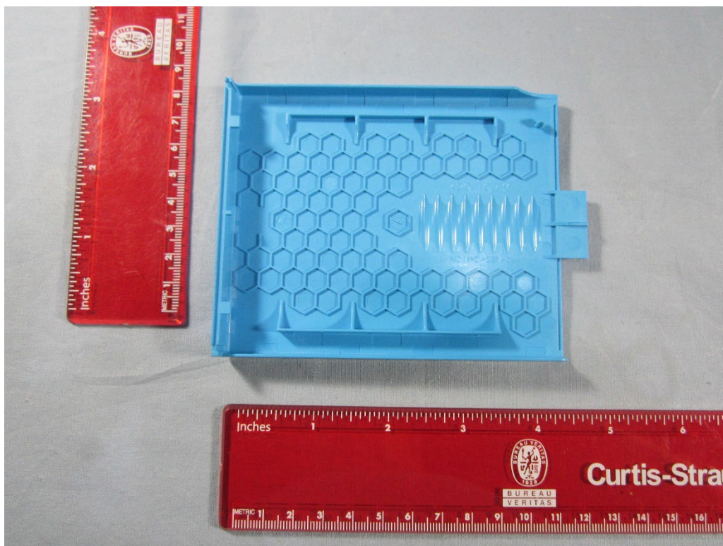
Back of Battery Cover
