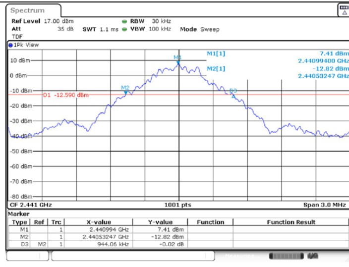
Middle Channel
