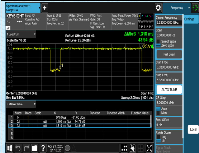
NTNV-11AC20SISO-Ant1-5320
