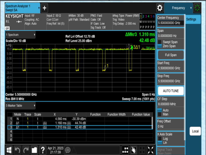
NTNV-11AC20SISO-Ant1-5500
