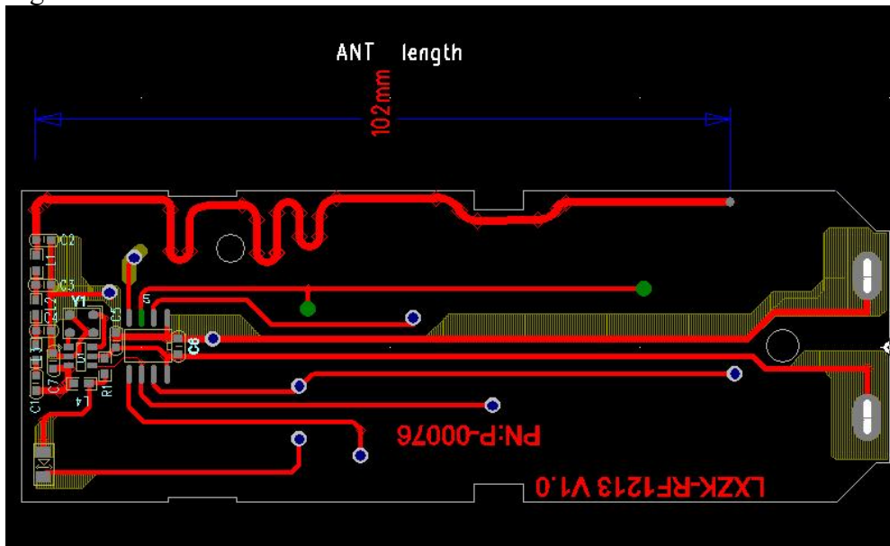
Fig.1: The dimension of the PCB Antenna
