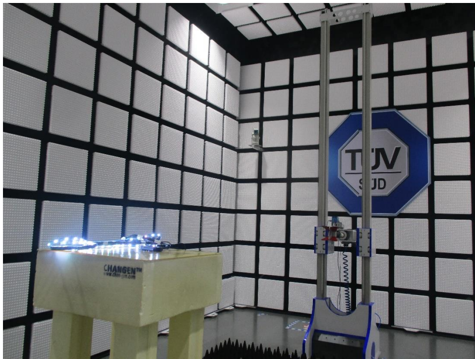
Radiated Emission test (2# Test Site) for 1-18GHz
