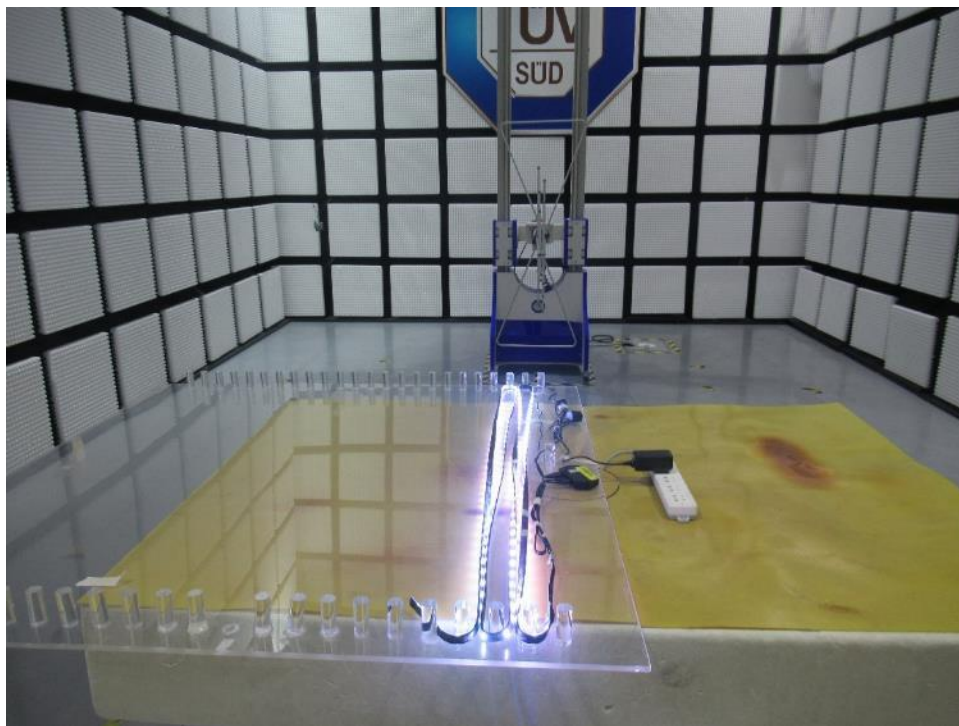
Radiated Emission test (1# Test Site) for 30MHz-1GHz
