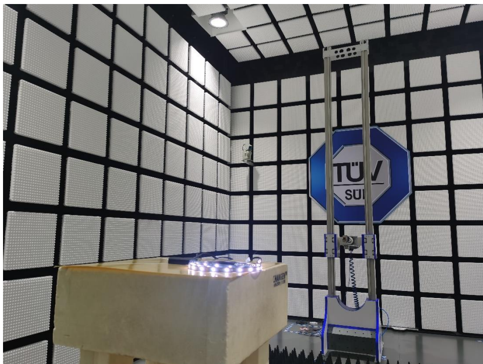
Radiated Emission test (2# Test Site) for 18-40GHz
