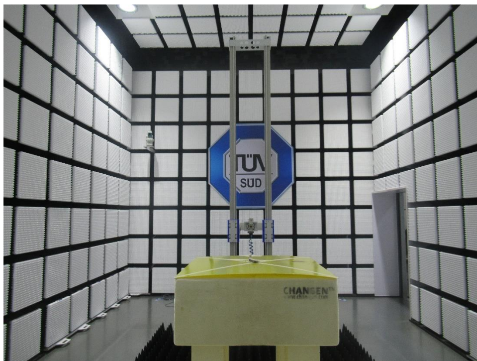
Radiated Emission test (2# Test Site) 18-40GHz
