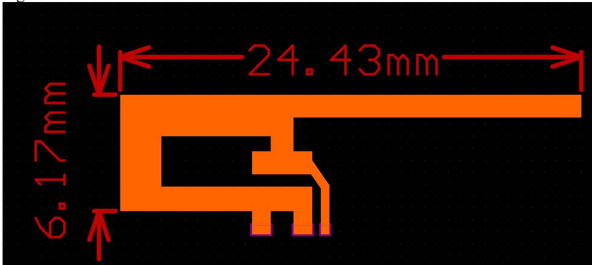
Fig.1: The dimension of the PCB Antenna
