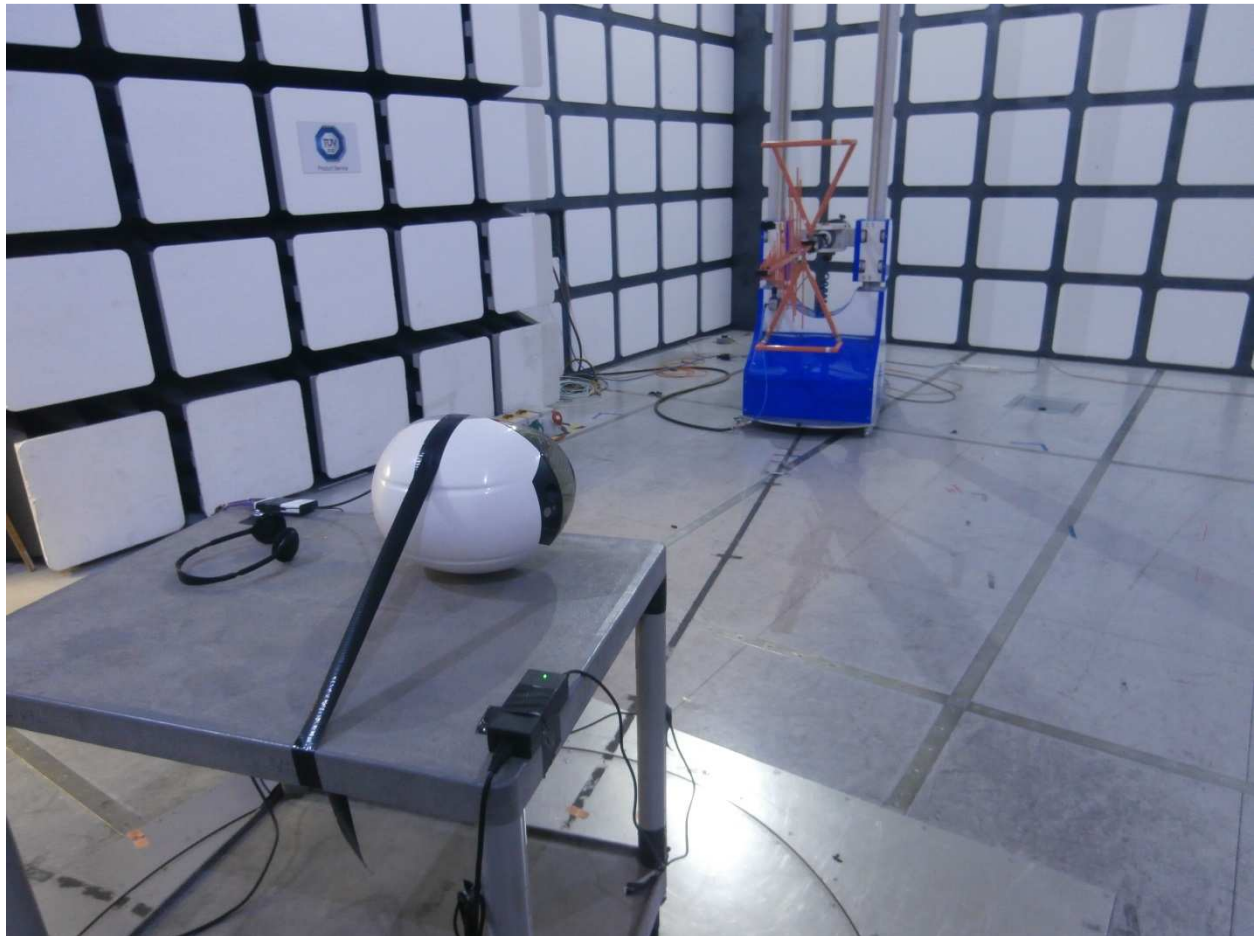
FCC Part Radiated Emissions 30 MHz to 1 GHz
