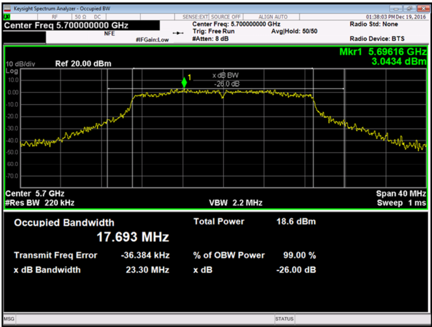
Figure 42 - U-NII 2c - 5700 MHz - 26 dB Bandwidth
