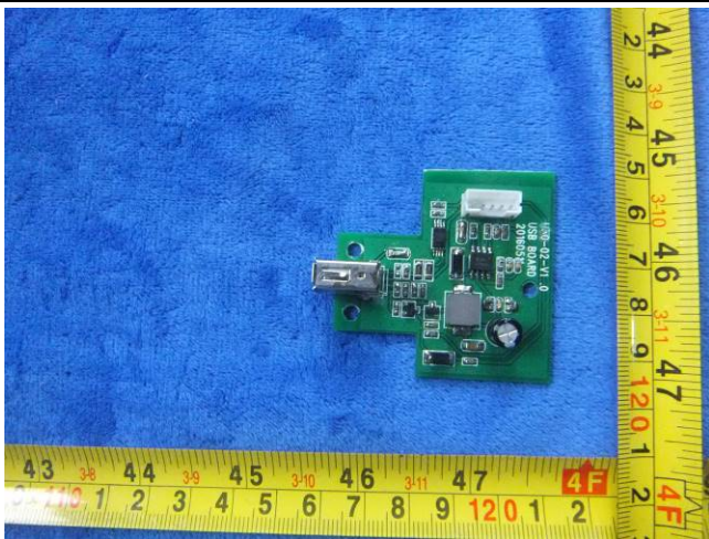
Sma1 Board 2 - Front View
