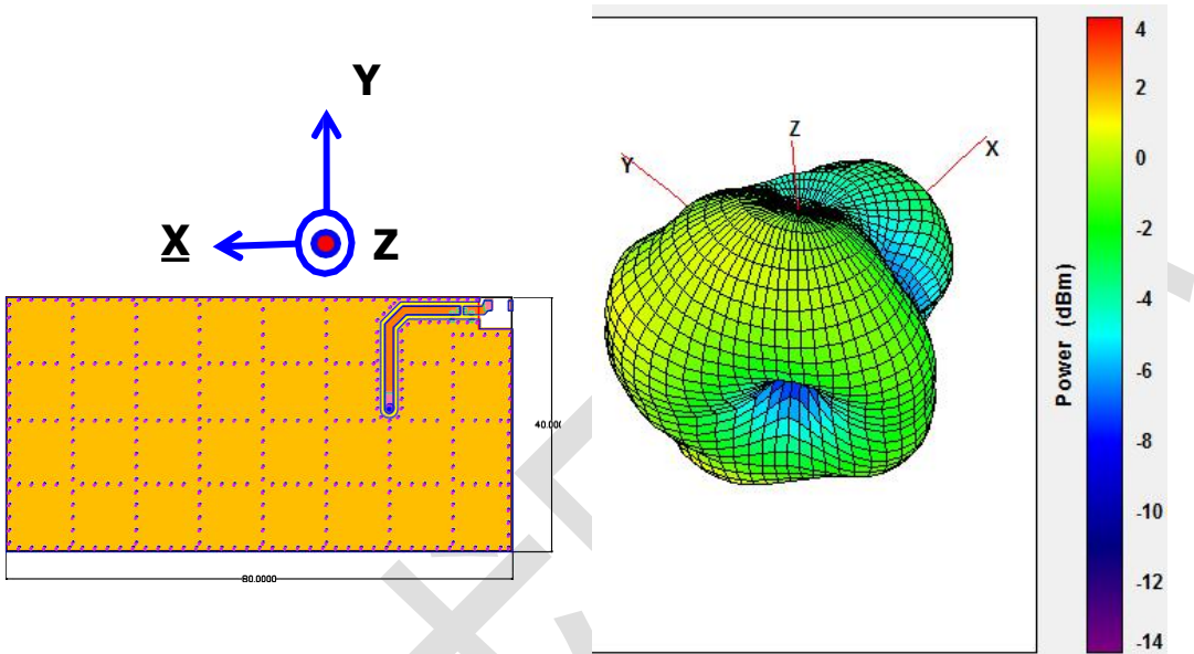
Radiation Pattern
