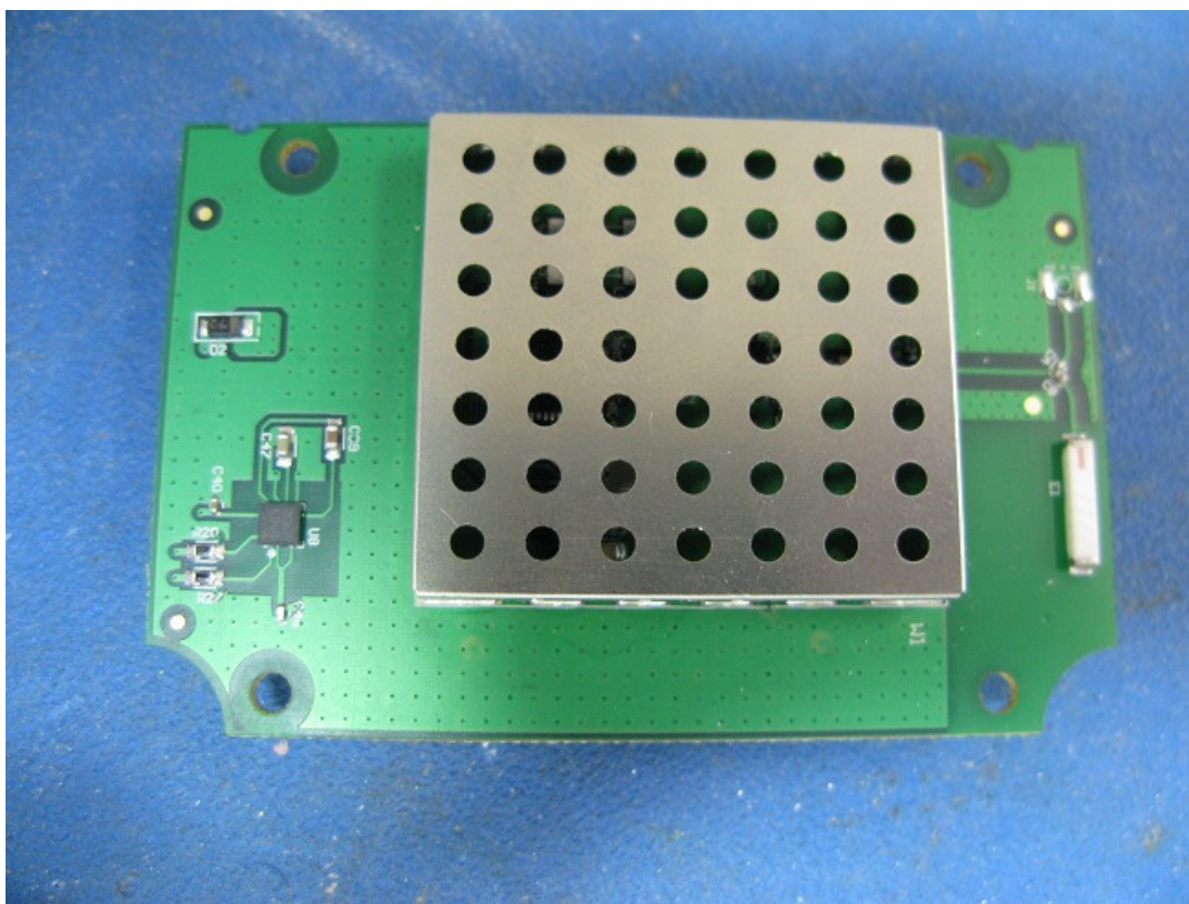
WASP Sensor Board with RF shield installed (top)
