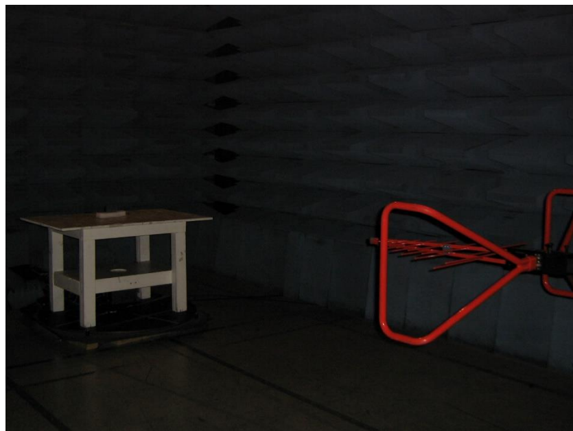
Radiated Emissions Setup in Semi-Anechoic Chamber, 30MHz-1GHz
